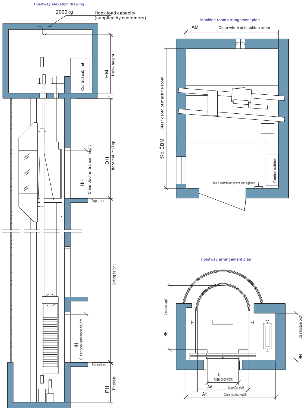
Main technical parameters (gearless)
