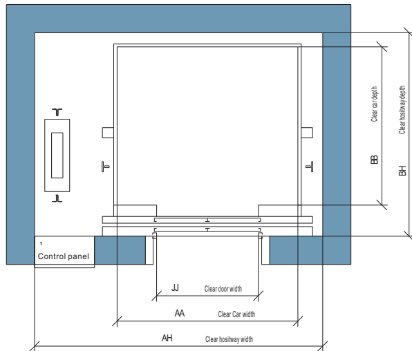
Hoistway arrangement plan
