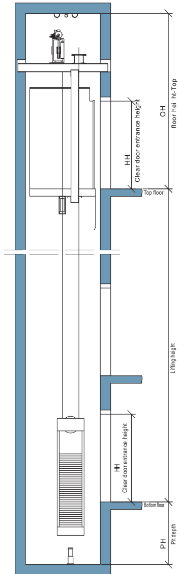
Hoistway elevation drawing
