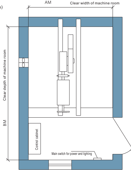
Machine room arrangement plan
