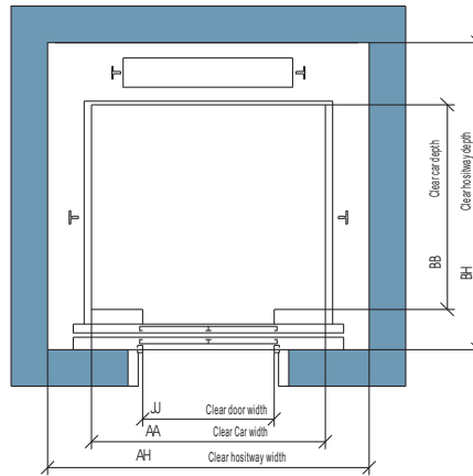
Hoistway ichnography
